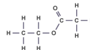
Ethyl ethanoate
